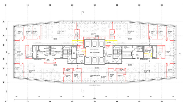
Layout plan
